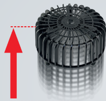
The idea: A leaf screen that raises itself mechanically when the backed up water level reaches 60 mm.
